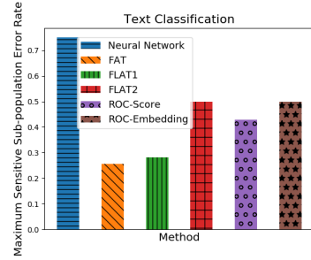
Figure 1: Comparison of maximum sub-population error rate on text classification
