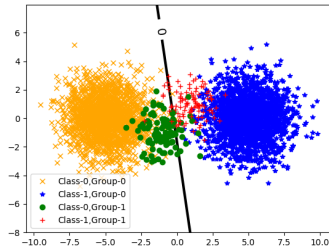
Figure 8: Decision boundary (black line) of Meta-fair classifier on synthetic dataset 2
