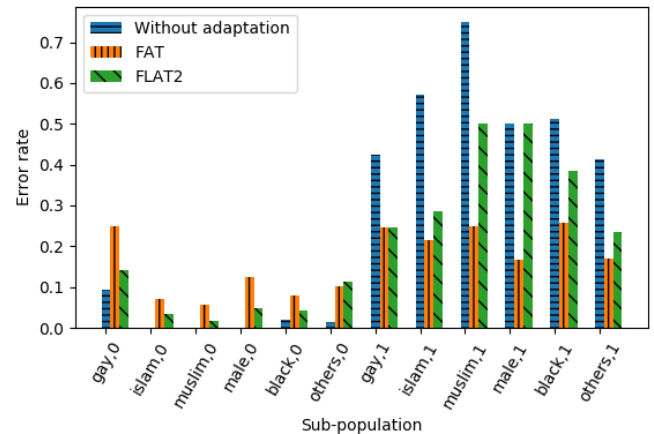
Figure 13: Group-wise class-wise error Rate on all sensitive sub-populations
